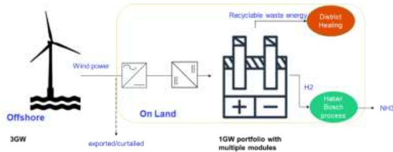
Figure 27. System model
