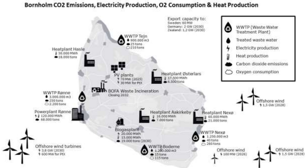
Figure 9. Mapping resources available in Bornholm for Power-to-X production.
