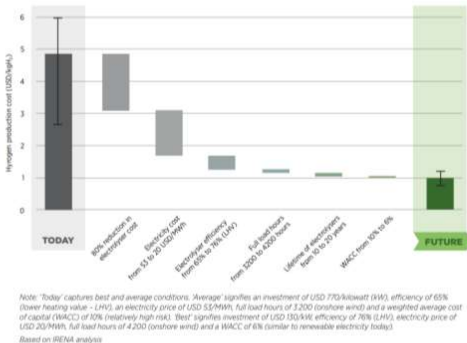
Figure 67. Potential to cut hydrogen cost from 2021 level to 2030 48
